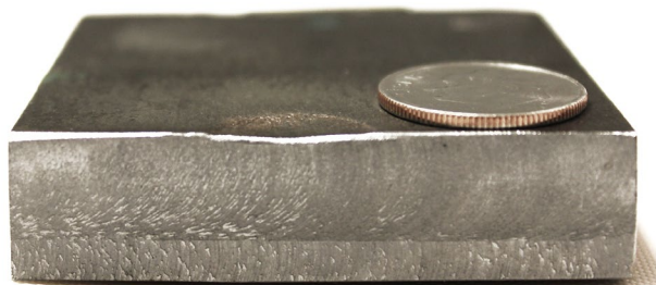
Tested for minimal impact at 0.25 in. (6.35 mm) standoff
